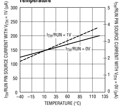
I_{TH}/RUN Pin Source Current vs Temperature
