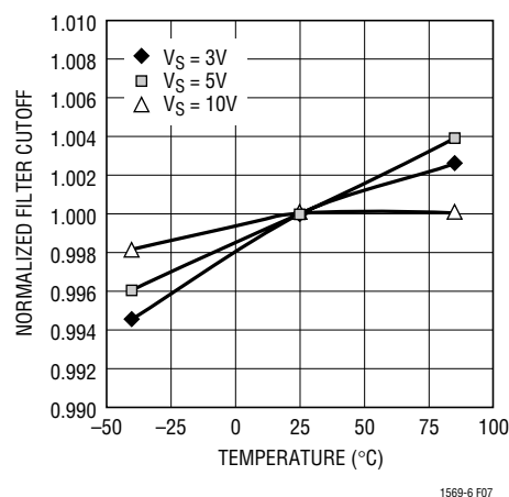
Figure 7. Filter Cutoff vs Temperature, Divide-by-16 Mode, R_{EXT} = 10k
