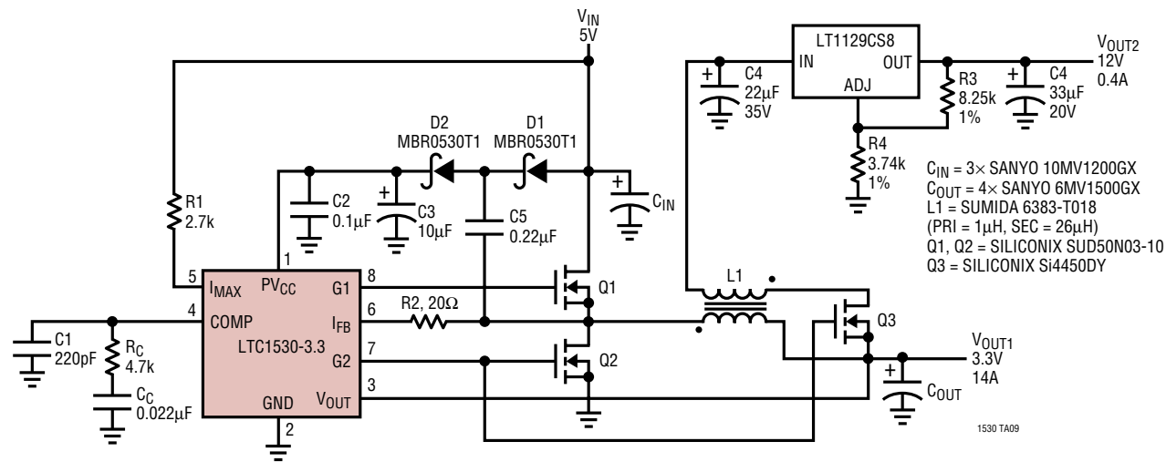
5V to Dual Output (3.3V and 12V) Synchronous Buck Converter
