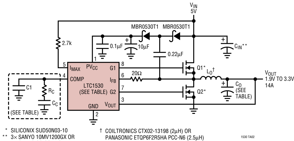
5V to 1.9V-3.3V Synchronous Buck Converter PV CC Is Generated from Charge Pump
