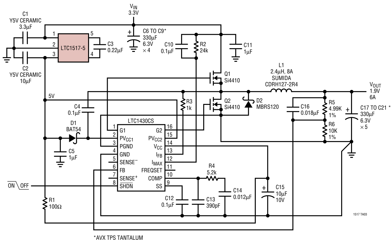
3.3V to 1.9V, 6A Power Supply
