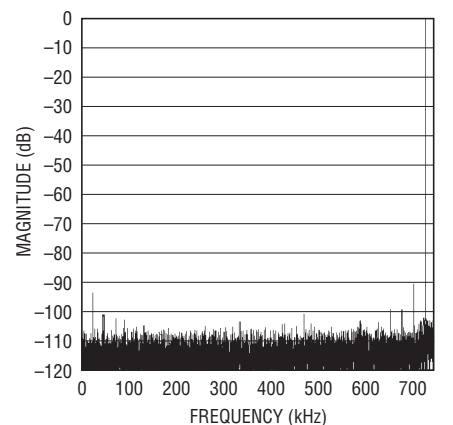
748kHz Sine Wave 4096 Point FFT Plot
