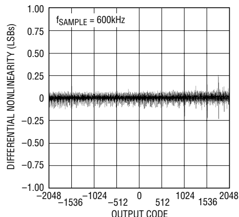
Bipolar Mode Differential Nonlinearity vs Output Code
