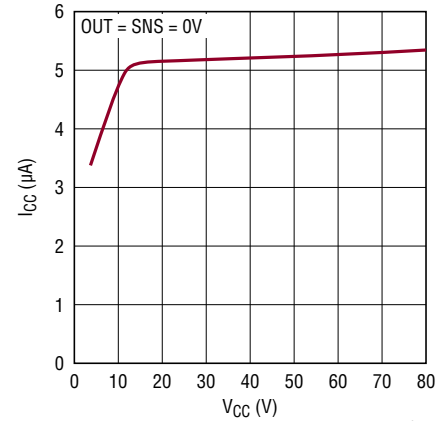
Supply Current During Shutdown vs Supply Voltage ( I_{CC}(SHDN) vs V_{CC} )
