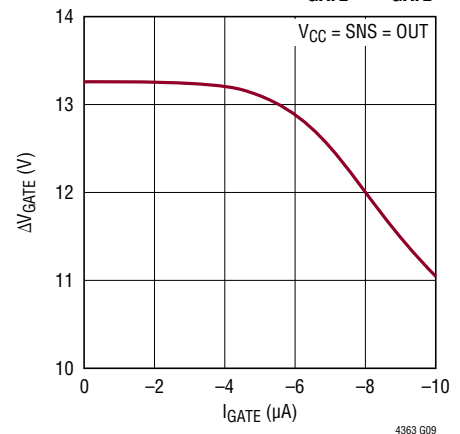
Gate Drive Voltage vs Gate Pull-Down Current \Delta V_{GATE} vs I_{GATE}
