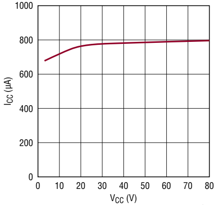
Supply Current vs Supply Voltage ( I_{CC} vs V_{CC} )
