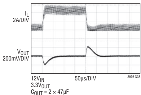
Load Transient: 0.5A to 4.5A
