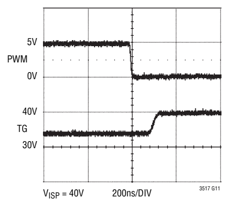
PMOS Turn-Off
