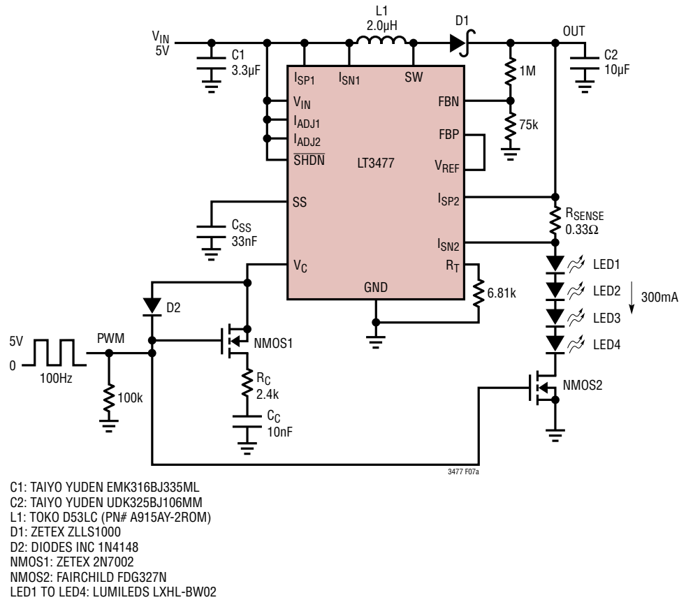
Figure 7a. 5V to 4 White LEDs: Boost With PWM Dimming
