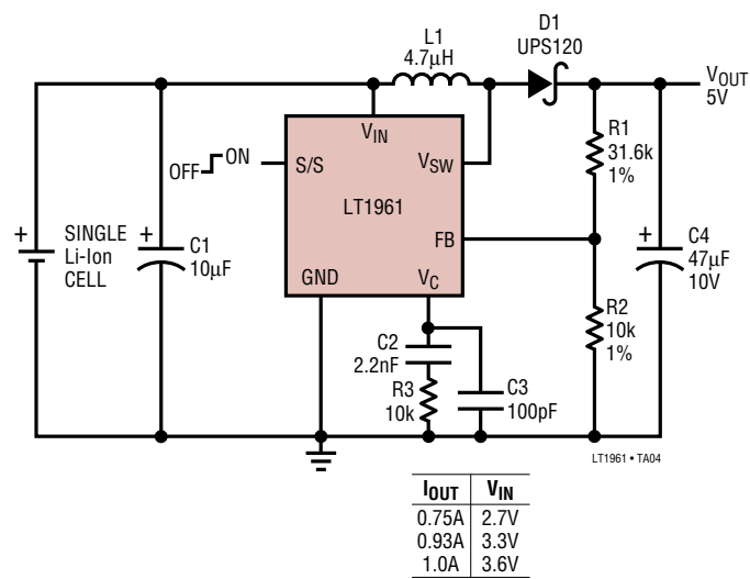
Single Li-Ion Cell to 5V
