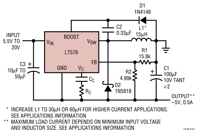
Figure 15. Positive-to-Negative Converter
