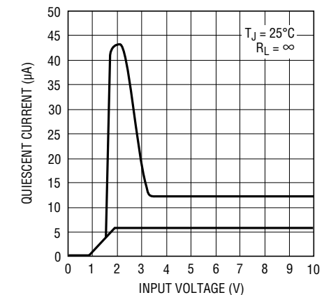
LT1521-3.3 Quiescent Current
