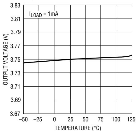
LT1521 Adjustable Pin Voltage
