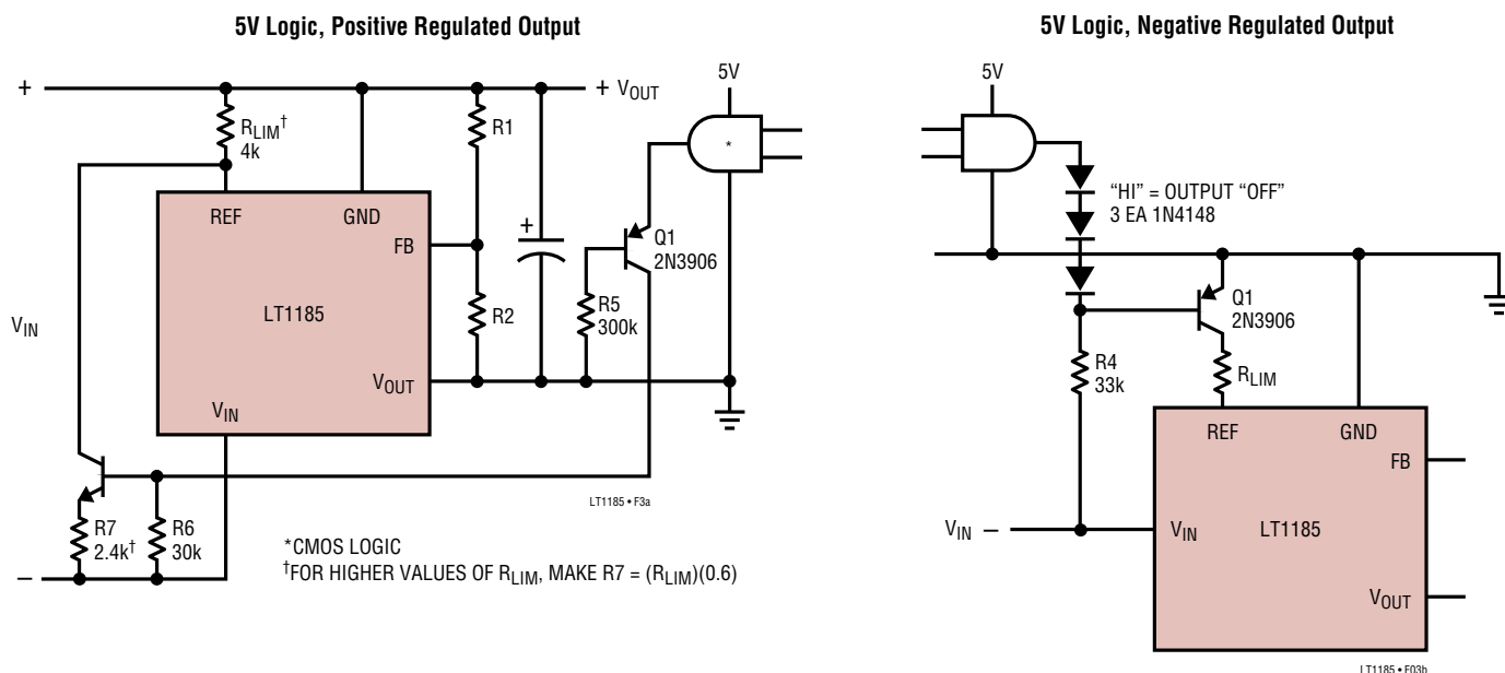
Figure 3. Shutdown Techniques
