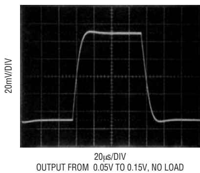
Small Signal Transient Response G = 10 , V_S = 5\text{V} , 0\text{V}
