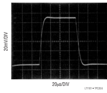
Small Signal Transient Response G = 10 , V_S = \pm 15\text{V}
