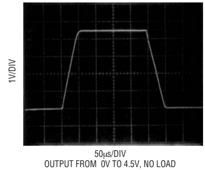
Large Signal Transient Response G = 10 , V_S = 5\text{V} , 0\text{V}
