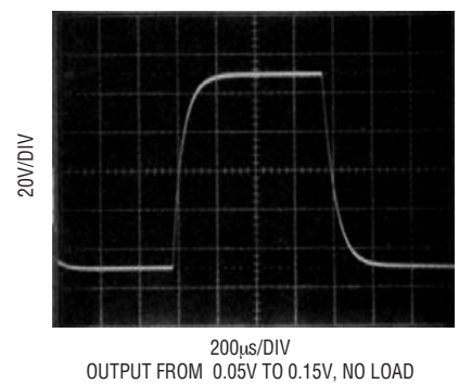
Small Signal Transient Response G = 100 , V_S = 5\text{V} , 0\text{V}
