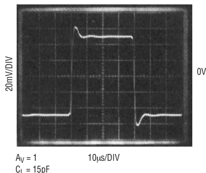
Small-Signal Transient Response V_S = \pm 2.5\text{V}
