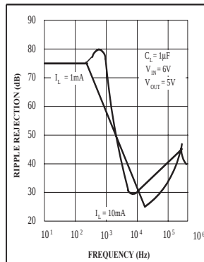
Ripple Rejection
