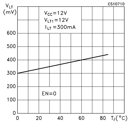
Figure 25: Loophrough Switch Drop Voltage vs Temperature
