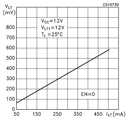
Figure 27: Loophrough Switch Drop Voltage vs Loophrough Current
