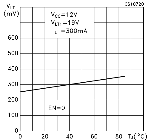
Figure 26: Loophrough Switch Drop Voltage vs Temperature
