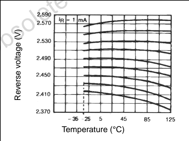
Figure 8. Temperature drift
