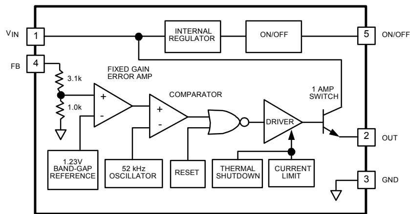
Fixed Regulator
