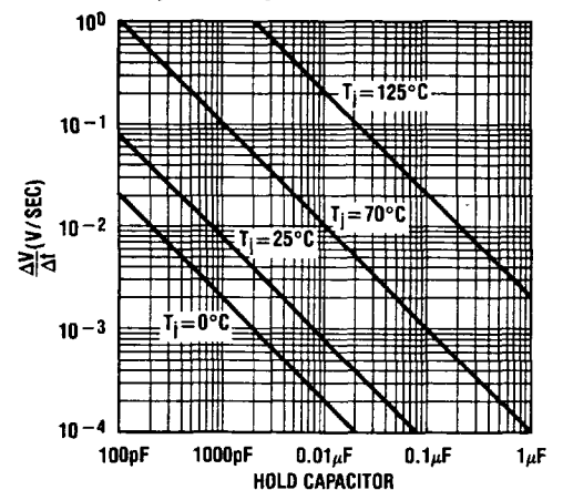
Output Droop Rate
