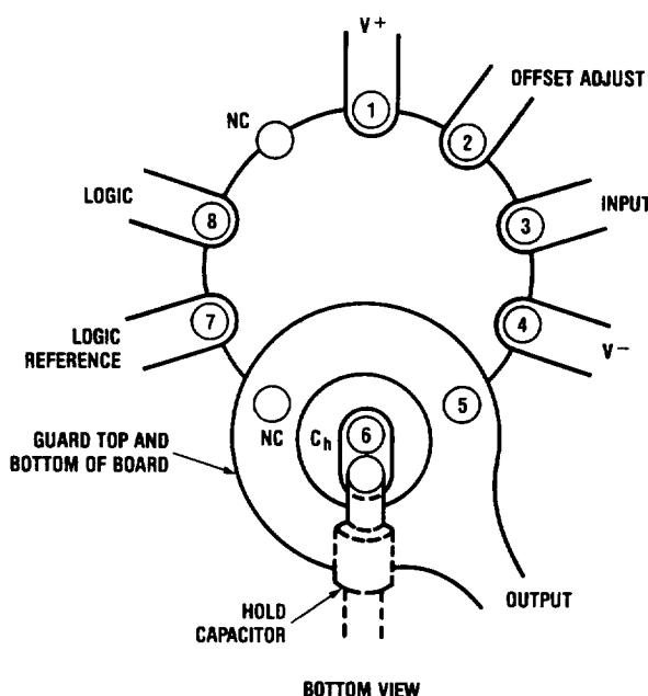
Guarding Technique
