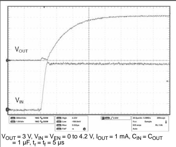
Figure 31. Startup transient
