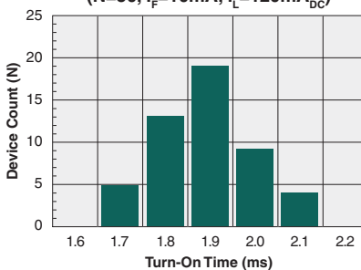
Typical Turn-On Time (N=50, I_F=10\text{mA} , I_L=120\text{mA}_{DC} )
