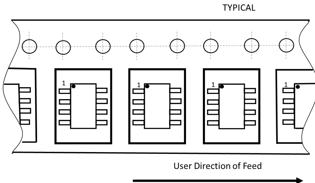
Figure 23. Tape orientation
