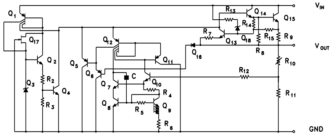
Figure 1. Schematic diagram
