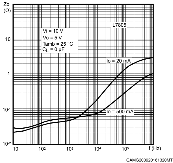
Figure 33. Output impedance vs frequency
