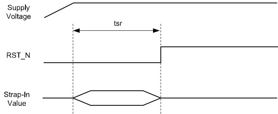
Figure 9. Reset Timing
