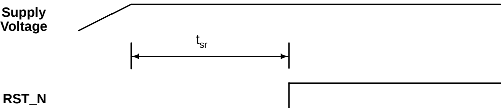
Figure 14. Reset Timing
