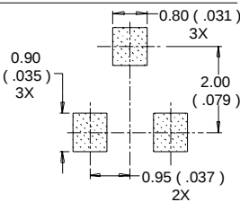
MINIMUM RECOMMENDED FOOTPRINT
