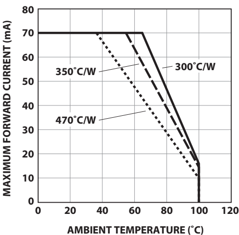
Figure 6: Maximum Forward Current vs. Ambient Temperature, Derated Based on T_{jmax} = 110^{\circ}\text{C} (AlInGaP)
