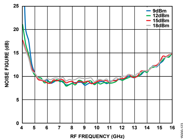
Figure 18. SSB Noise Figure vs. RF Frequency at Various LO Powers, IF = 100 MHz
