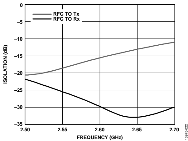
Figure 21. Isolation vs. Frequency
