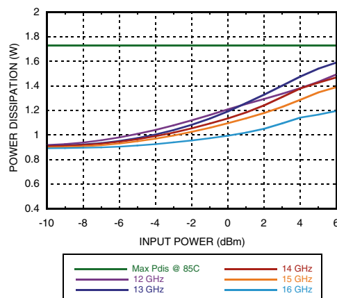
Power Dissipation
