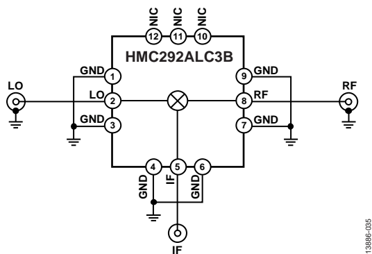
Figure 35. Typical Application Circuit
