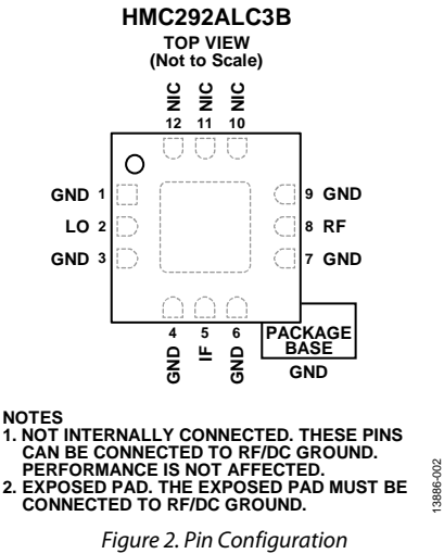
Figure 2. Pin Configuration
