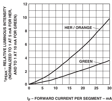
Figure 9. Relative luminous intensity vs. dc forward current.
