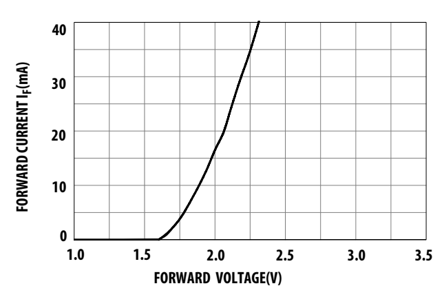
Figure 16: Forward Current vs. Forward Voltage
