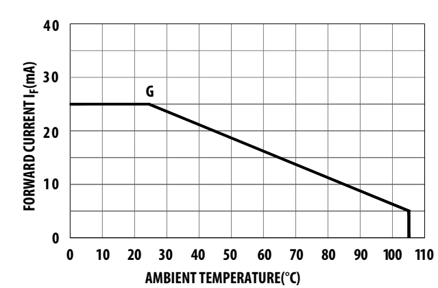
Figure 3: Allowable DC Current vs. Ambient Temperature
