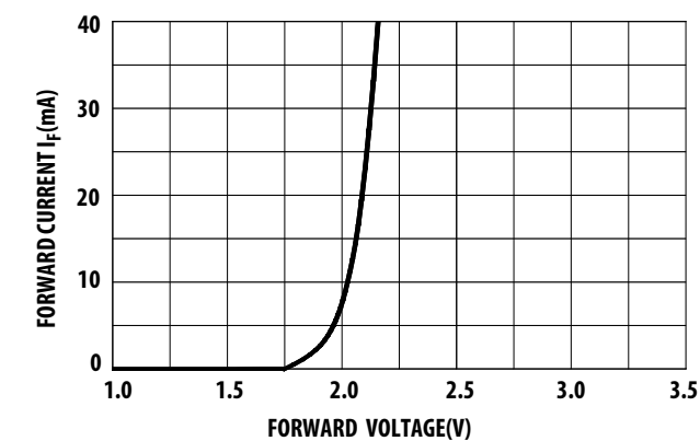
Figure 8: Forward Current vs. Forward Voltage
