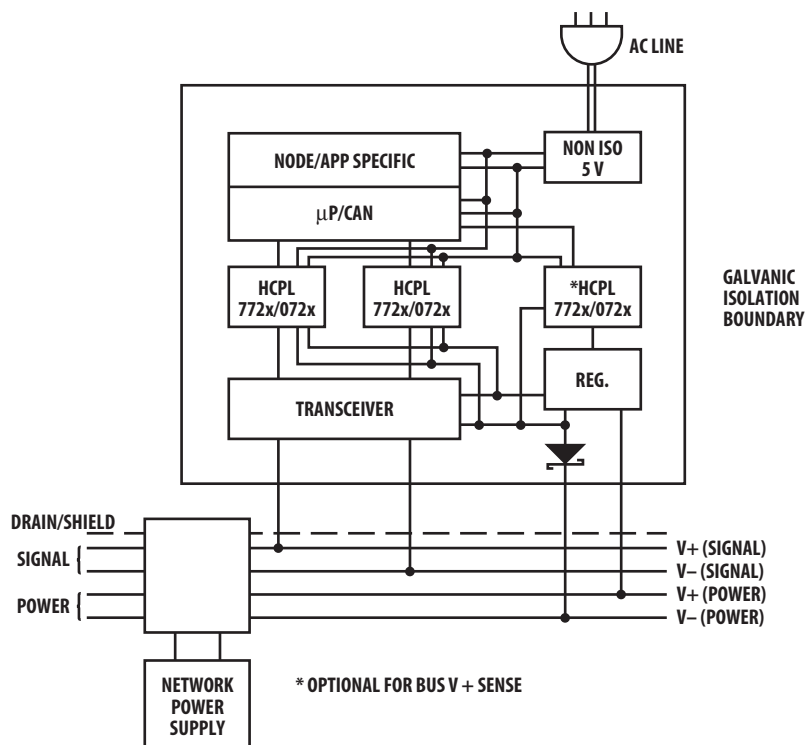
Figure 15: Isolated Node with Transceiver Powered by the Network
