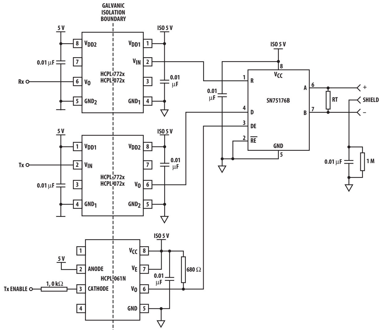
Figure 19: Recommended PROFIBUS Application Circuit
