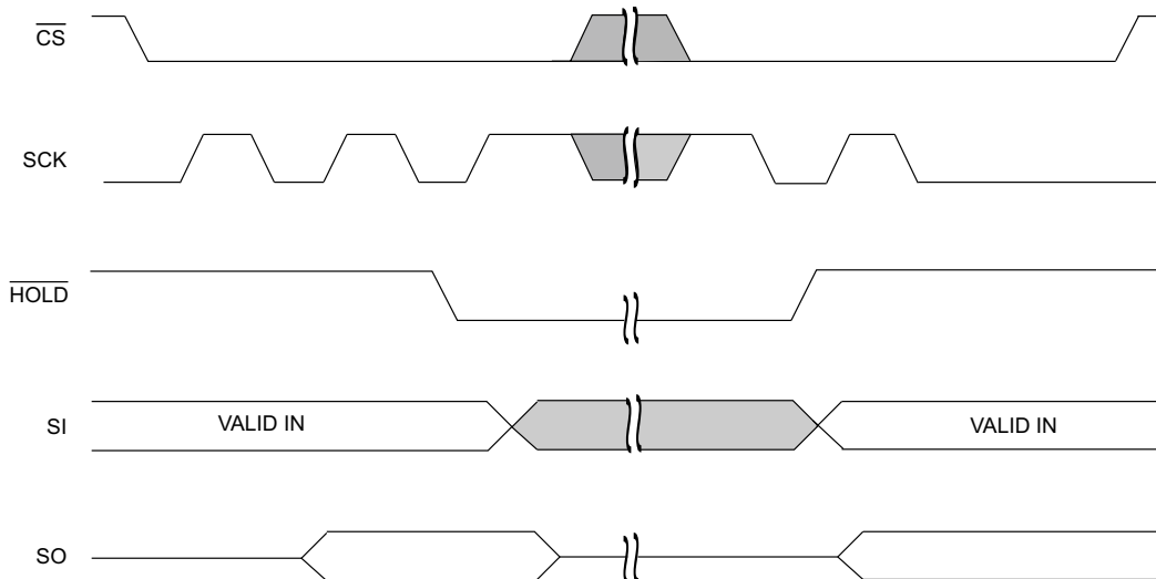
Figure 13. HOLD Operation [2]
