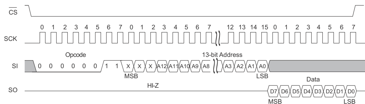
Figure 12. Memory Read
