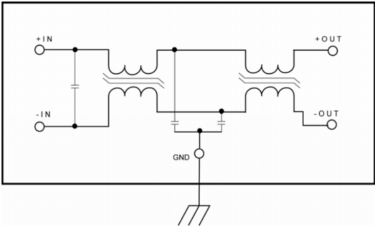
Figure 7 - Filter Block Schematic
