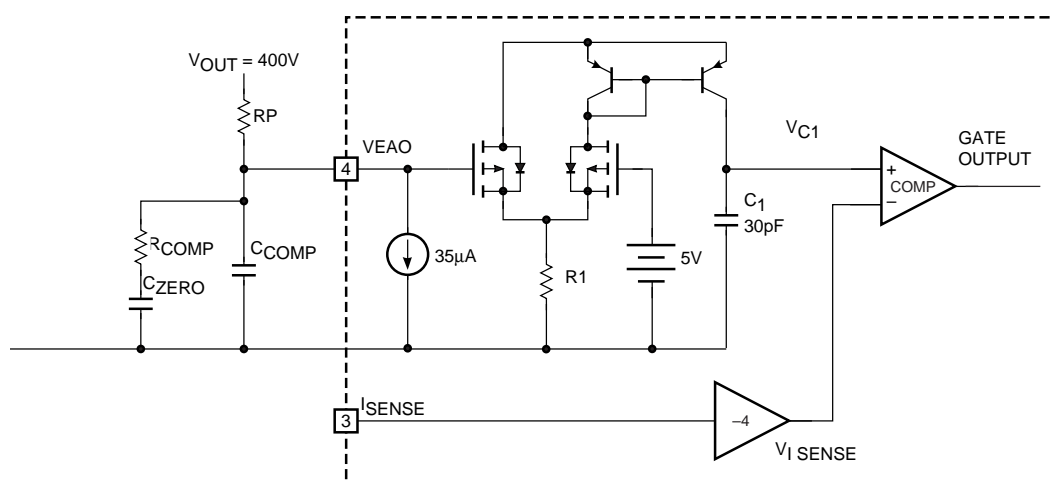
Figure 11. FAN4803 PFC Control
