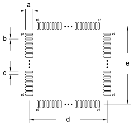
Figure 10.2. TQFP48 PCB Land Pattern
