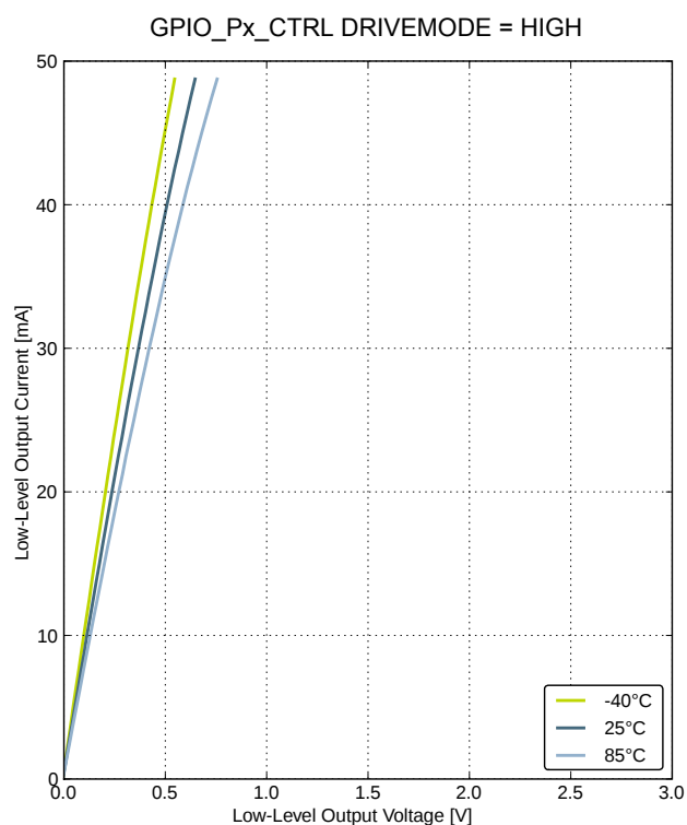
Figure 4.6. Typical Low-Level Output Current, 3 V Supply Voltage
