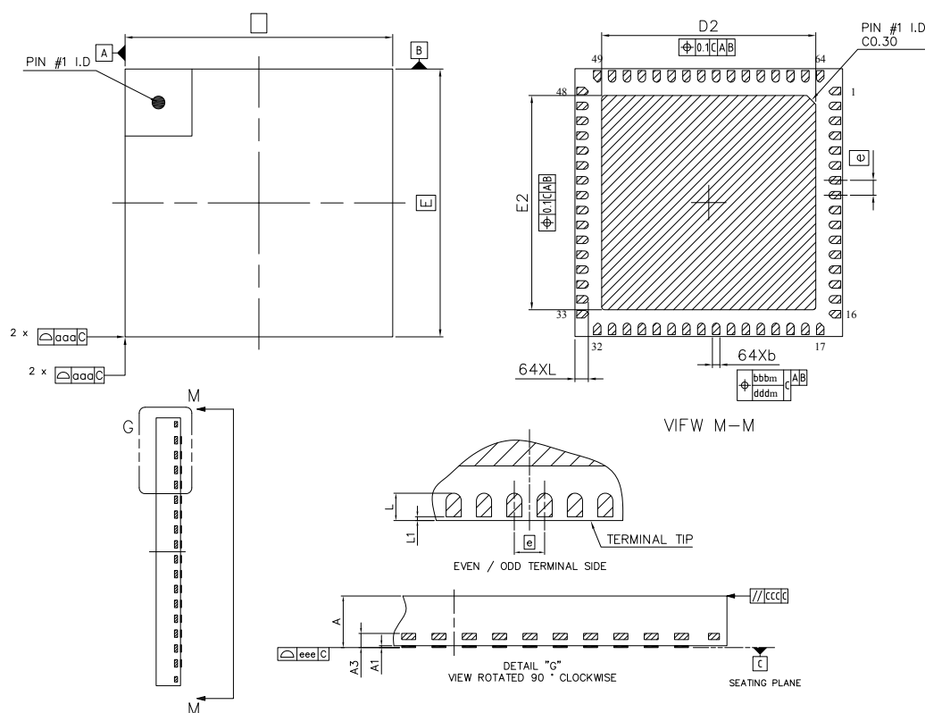
Figure 9.1. QFN64
