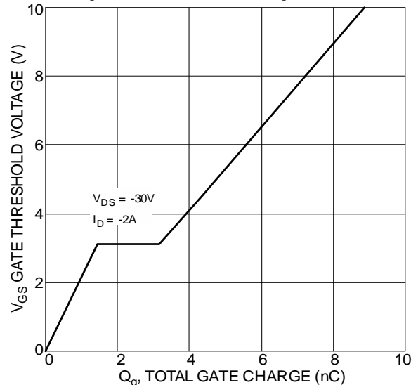
Figure 23 Gate Charge
