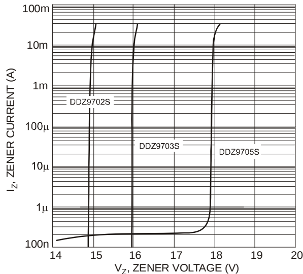
Fig. 6 Typical Zener Breakdown Characteristics, DDZ9702S - DDZ9705S
