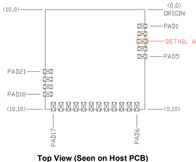
Figure 6. Solder Pad Reference Location
