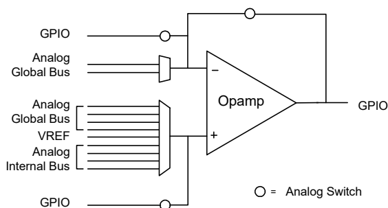
Figure 8-6. Opamp
