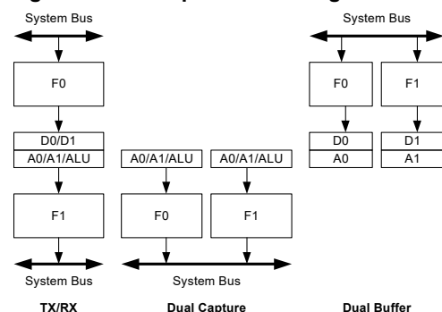
Figure 7-5. Example FIFO Configurations
