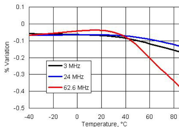
Figure 11-71. IMO Frequency Variation vs. Temperature
