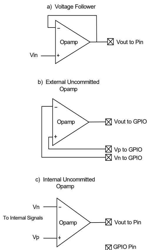
Figure 8-7. Opamp Configurations
