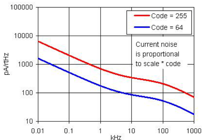
Figure 11-49. IDAC Current Noise, 255 \mu A Mode, Source Mode, High speed mode, V_{DDA} = 5 V
