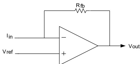
Figure 8-9. Continuous Time TIA Schematic
