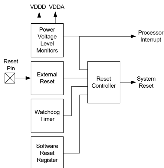
Figure 6-8. Resets
