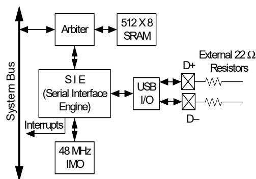
Figure 7-16. USB
