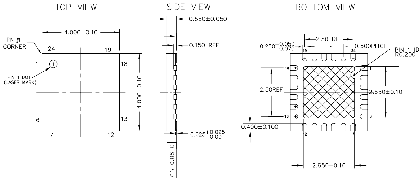
Figure 18. 24-Pin (4 × 4 × 0.6 mm) QFN
