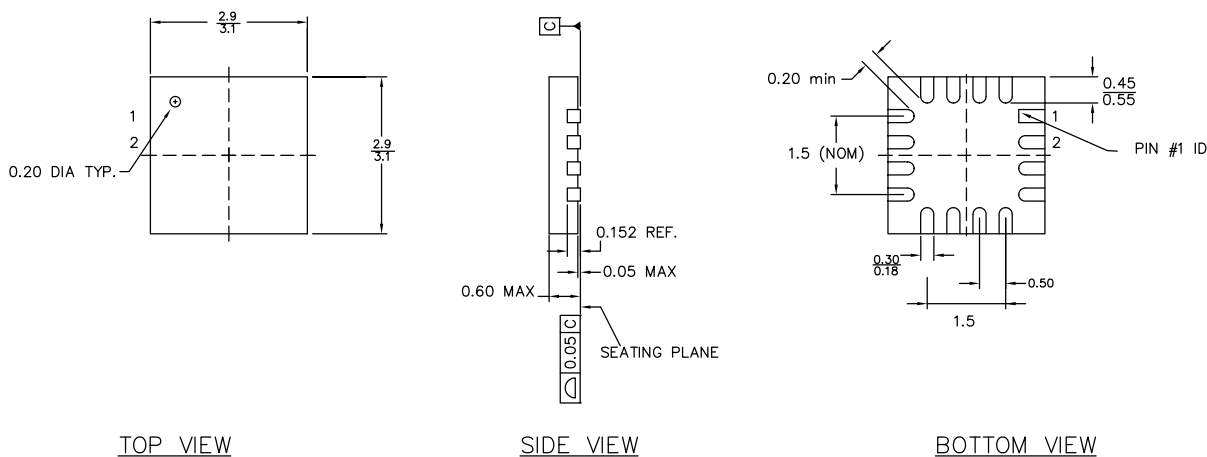
Figure 17. 16-pin QFN No Center Pad (3 x 3 x 0.6 mm) Package Outline (Sawn)
