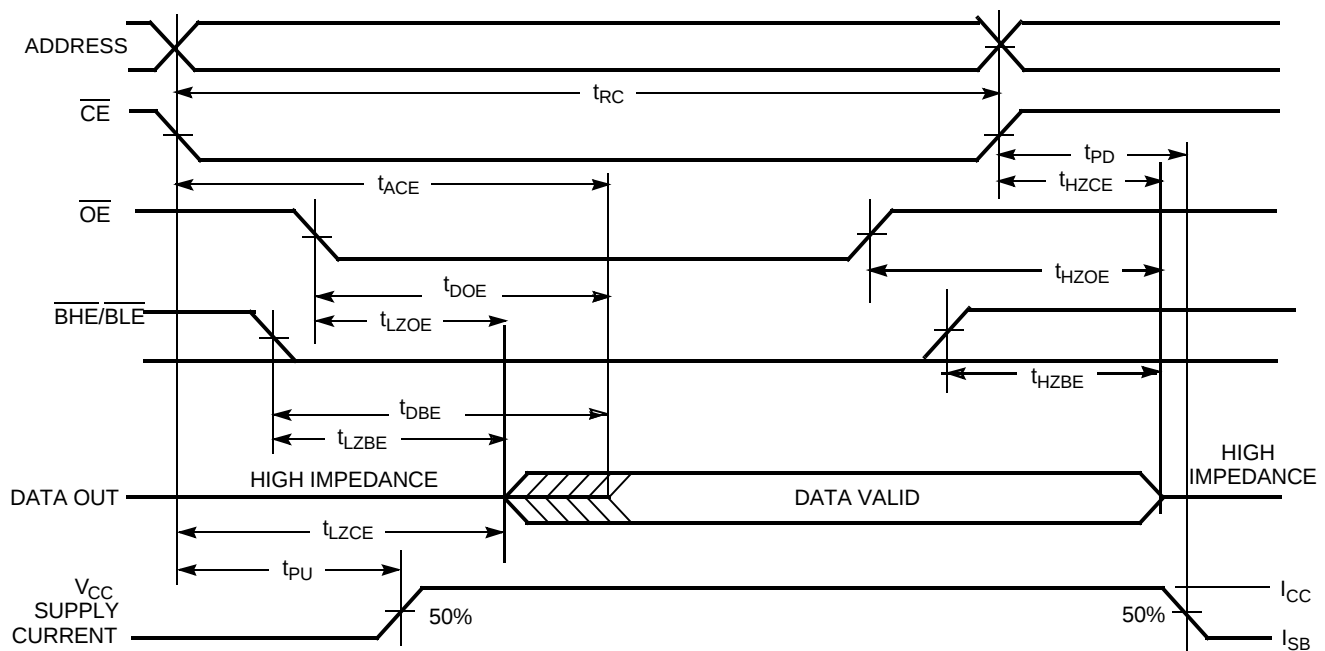
Figure 6. Read Cycle No. 2: \overline{\text{OE}} Controlled [22, 23]
