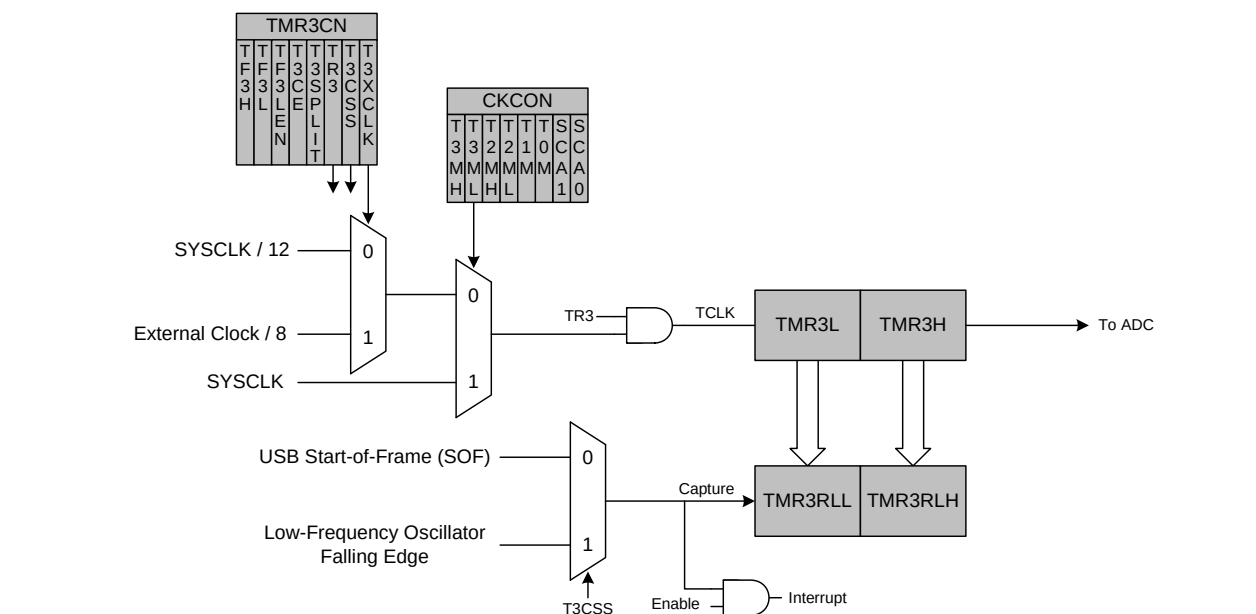
Figure 21.10. Timer 3 Capture Mode (T3SPLIT = '0')
