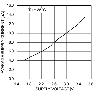
Fig.41 I_{DD} - Supply voltage
