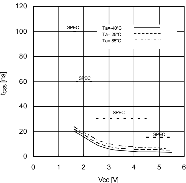
Figure 24. CSB Setup Time vs Supply Voltage
