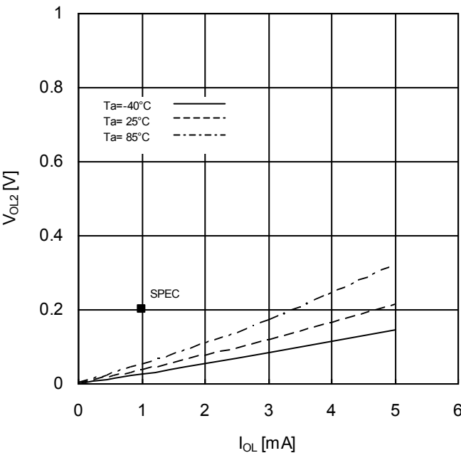
Figure 8. Output Low Voltage2 vs Output Current (Vcc=1.6V)
