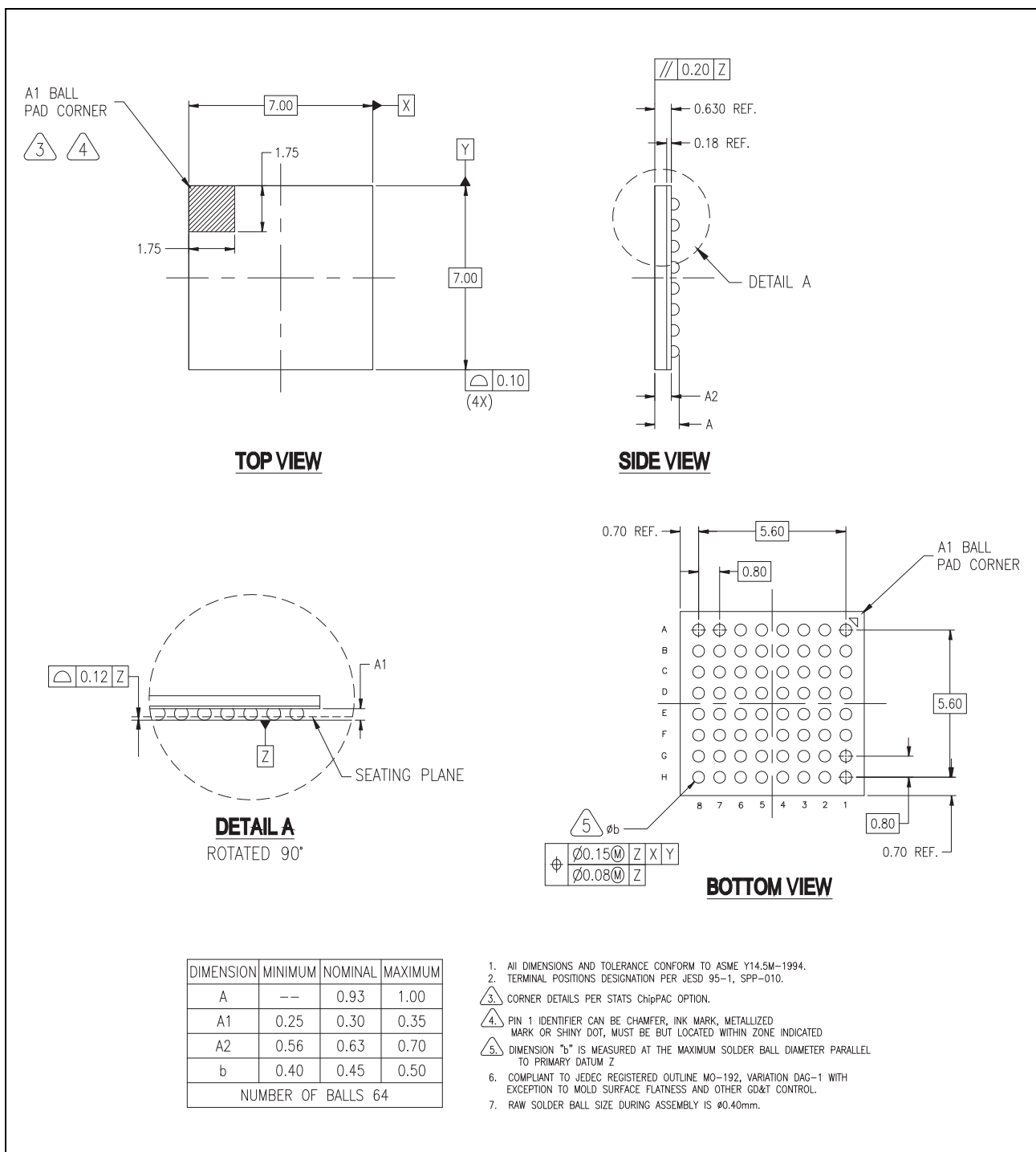
Figure 17: 64-pin FBGA Package
