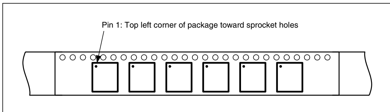
Figure 18: Pin 1 Orientation
